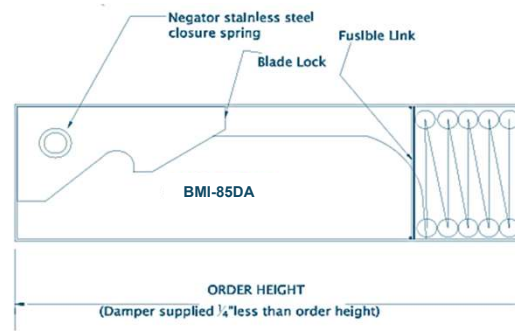
(H) HORIZONTAL MOUNT
